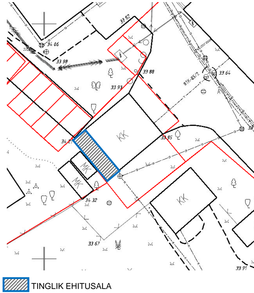
TURU TN 21B PTH-13-267 LISA EHITUSALA SKEEM
